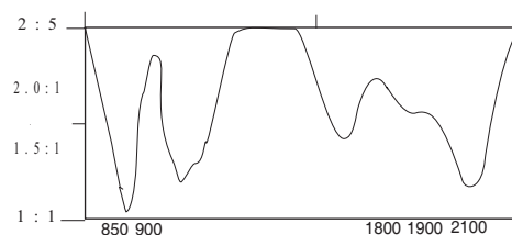
TYPICAL VSWR PATTERN (NOT TO SCALE)
